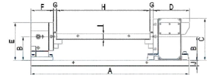
Fixture Plate
